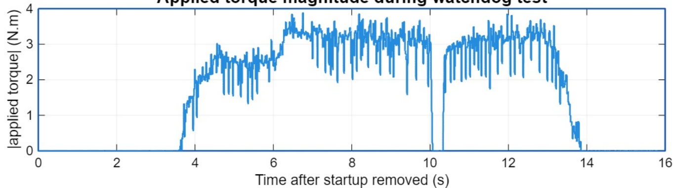
Applied torque magnitude during watchdog test
